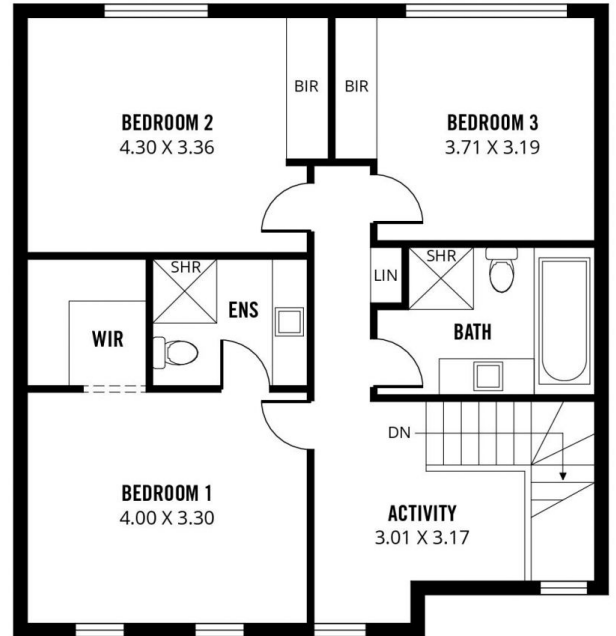
UPPER FLOOR
